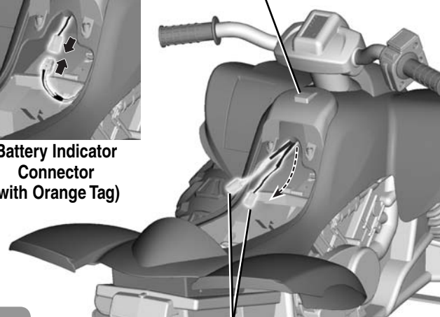
Connectors
