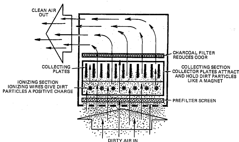
FIG. 1 Pictorial Illustration of Air Cleaning Process
