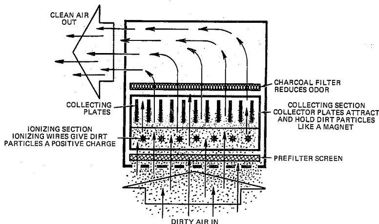
FIG. 1 Pictoral Illustration of Air Cleaning Process
