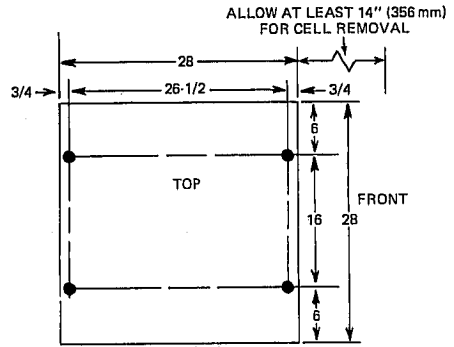
FIG. 2 - Approximate Installation Dimensions in inches.
