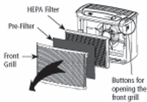
Figure 1 - Models 30117, 30119 & 30145
