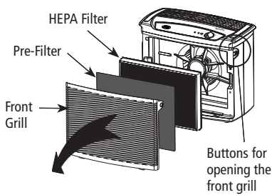
Figure 1 - Models 30117, 30119 & 30145
