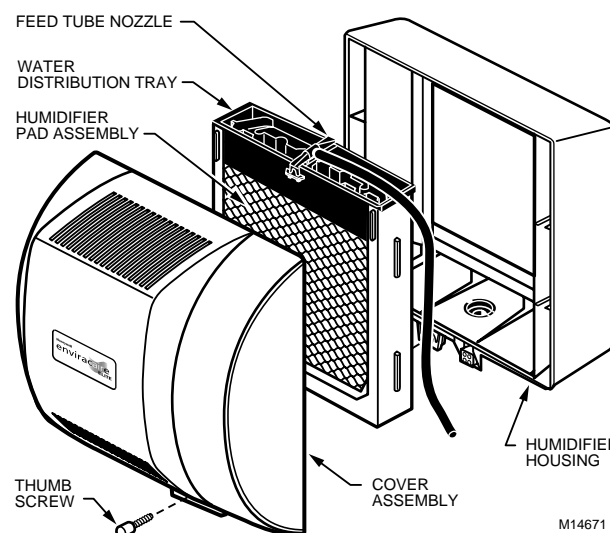
Fig. 3. Humidifier components.
