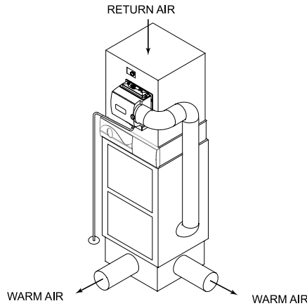
COUNTER-FLOW
