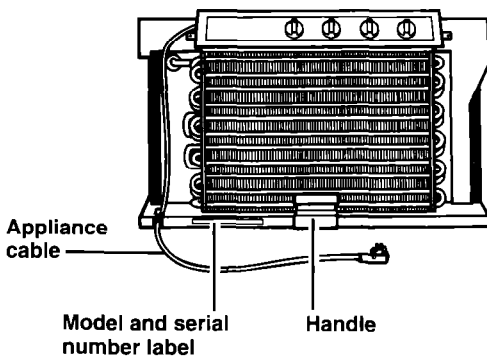
Front view of unit with front panel removed
