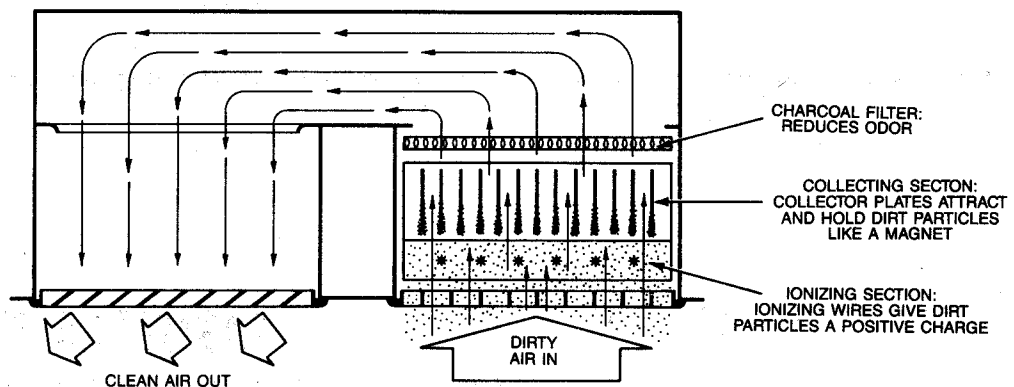
FIG. 1 Pictorial Illustration of Air Cleaning Process
