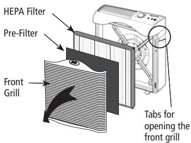
Figure 1 - Models 30090 & 37090
