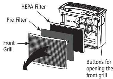
Figure 2 - Model 30105
