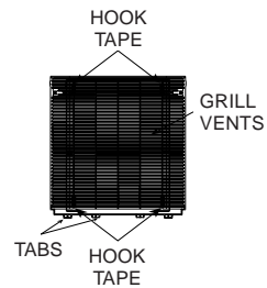
Fig. 3 - Inside Surface of Front Grill
