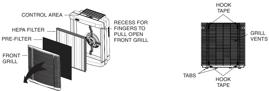
Fig. 2 - Air Purifier Components
