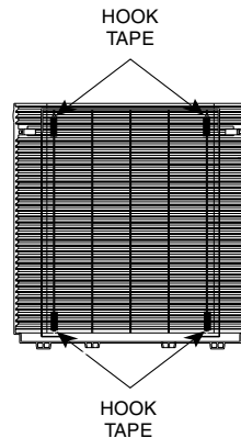
Fig. 3 - Inside Surface of Front Grill
