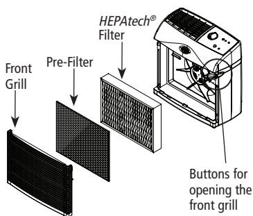
Figure 1 - Model 30057A
