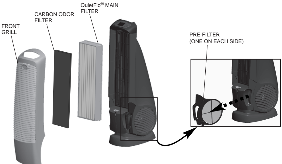
Fig. 2 - Air Purifier Components
