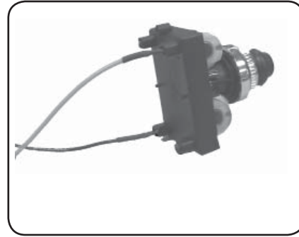
Fig. 16-2 Spark generator
