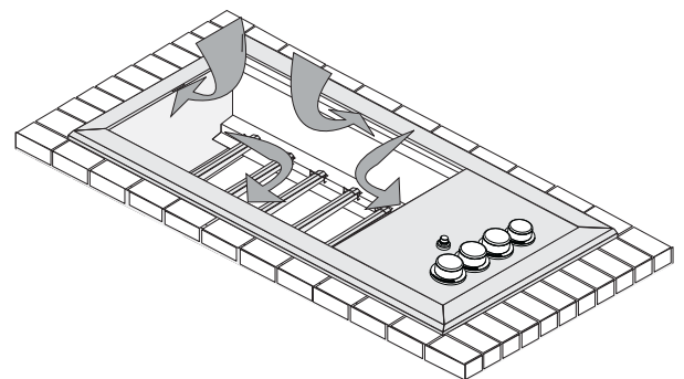
Fig. 10-1 - Ventilation Diagram
