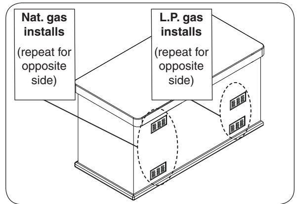
Fig. 11-1 Ventilation detail
