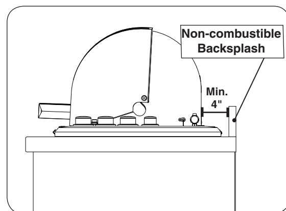
Fig. 9-4 Backsplash clearance
