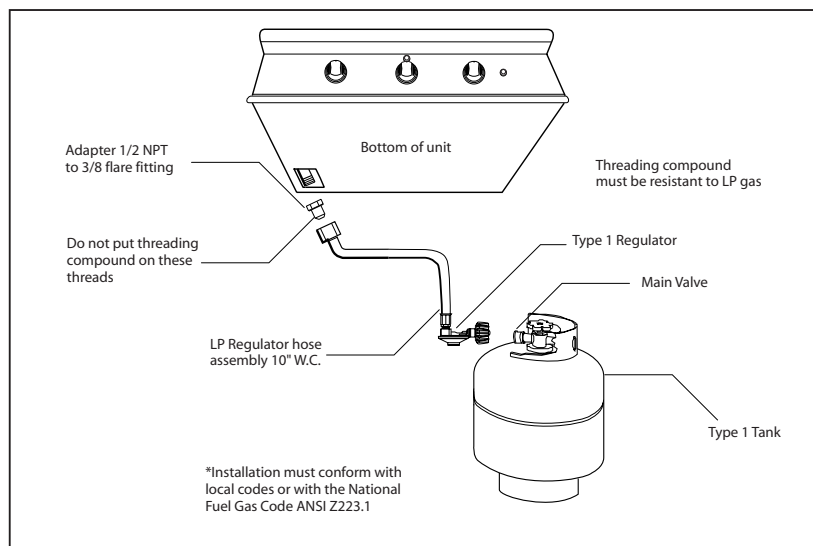
FIG.02 LP Gas (27BQR Shown)
