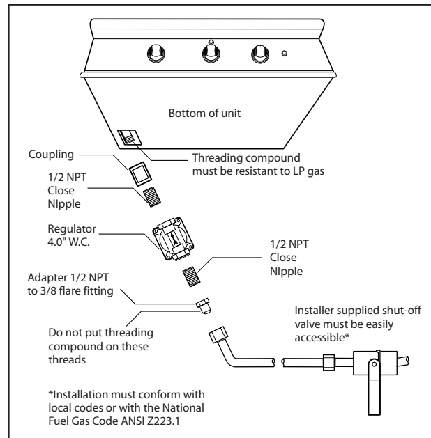
FIG.01 Natural Gas (27BQR Shown)
