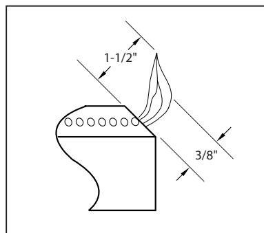
FIG.9 Power Burner Flame Height
