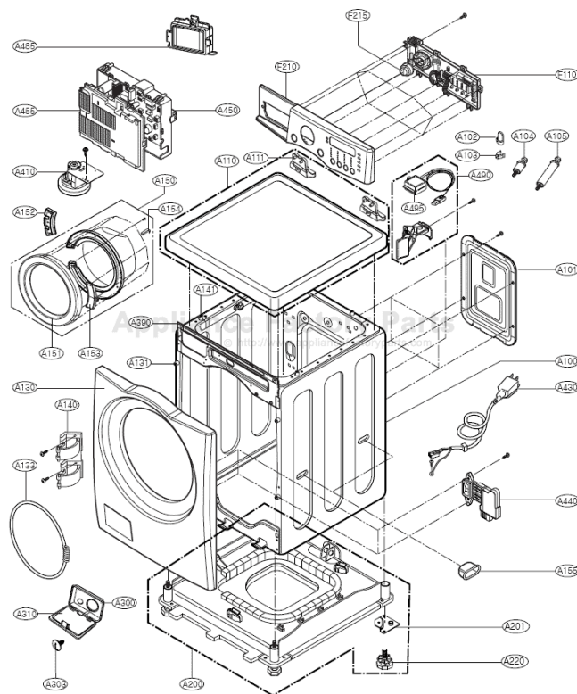
10-1. CABINET & CONTROL PANEL ASSEMBLY
