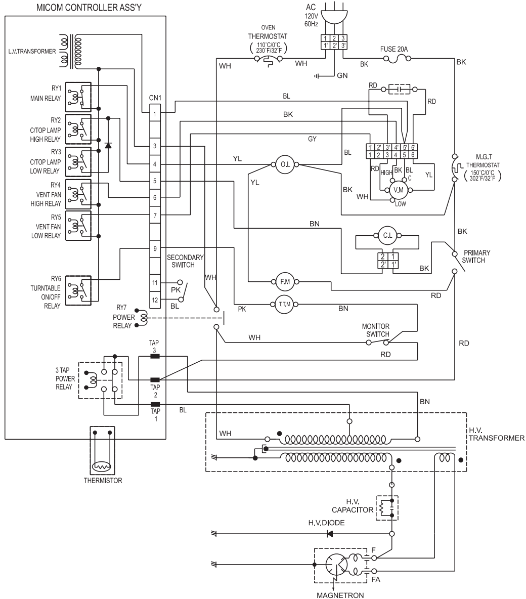
CONTROL MODULE
