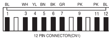
CONTROL MODULE
