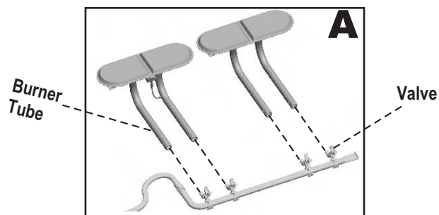
Correct burner-to-valve engagement
