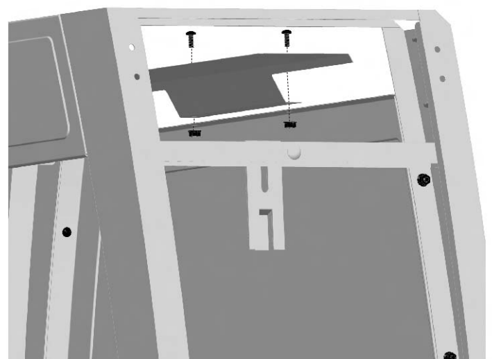
Back view of heat shield
