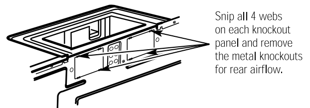
Oven Rear Panel
