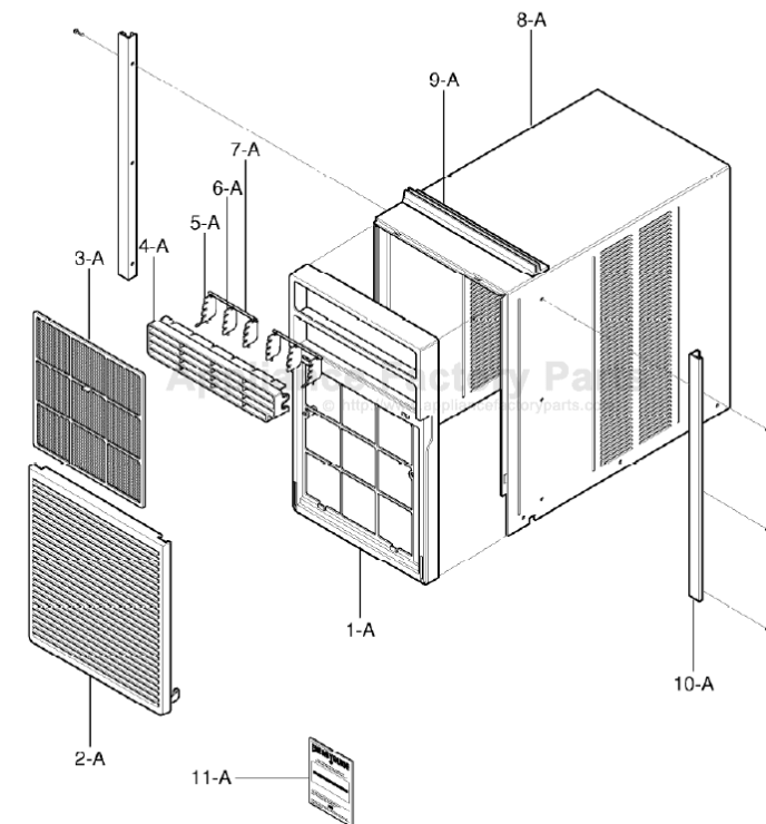
CABINET & FRONT GRILLE ASSEMBLY
