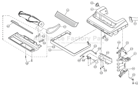
Nozzle Housing
