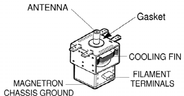
MAGNETRON
