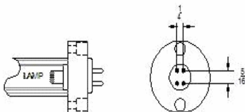
TYPICAL T3 LAMP 4 PIN CELL BASE
