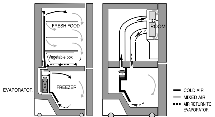
AIR FLOW
