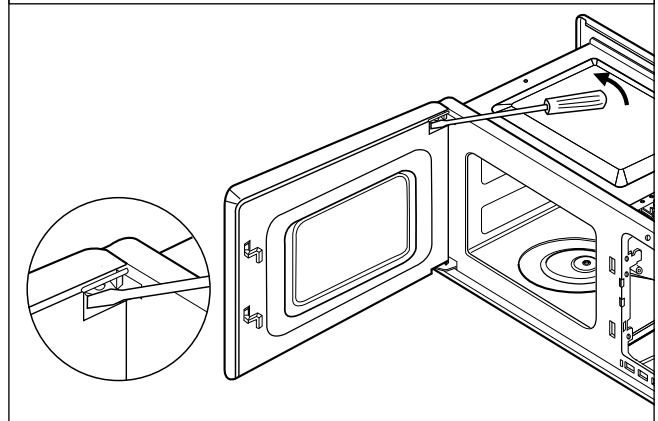
Remove choke cover
