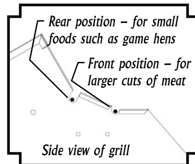
Figure 16-2 - Dual position rotisserie system.
