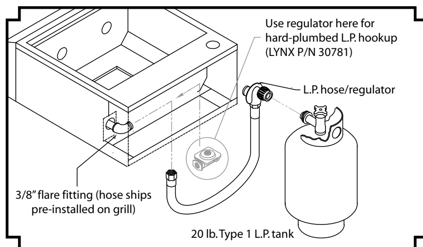
Figure 9-1 - Typical attachment to L.P. tank.
