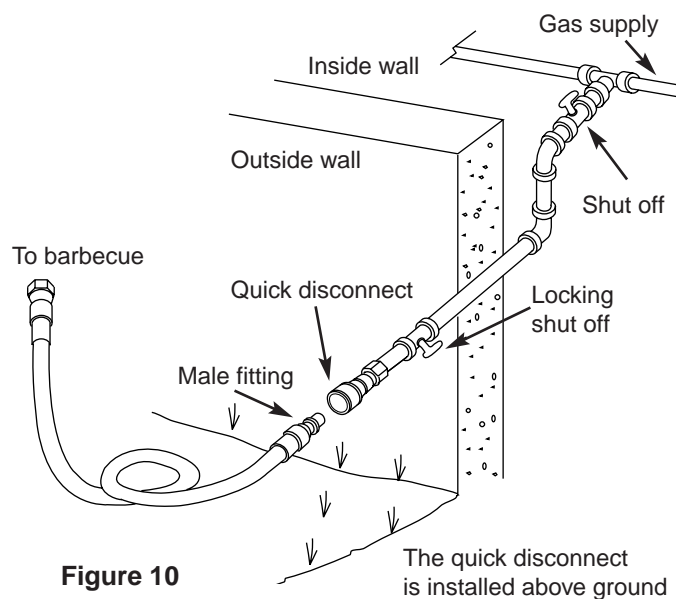
Typical natural gas supply installation. Figure 10.
