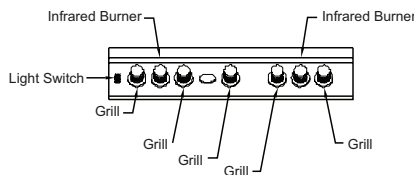
Five Burner Grill
