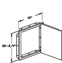
SINGLE ACCESS DOOR FRONT DIMENSIONS
