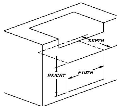
SINGLE ACCESS DOOR REAR CUT OUT DIMENSIONS
