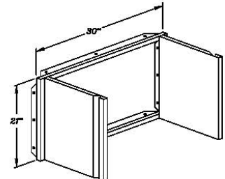
DOUBLE ACCESS DOOR FRONT DIMENSIONS
