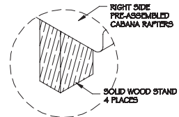
VIEW-B SOLID WOOD STANDS USE SOLID WOOD STANDS TO STABILIZE AND SUPPORT PRE-ASSEMBLED CABANA RAFTERS (FOUR PLACES.)
