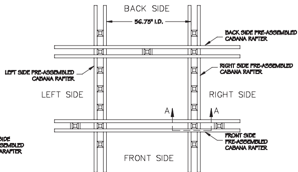
TOP VIEW WIRING CABANA RAFTERS
