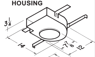
MODEL 503 HOUSING
