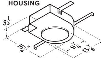
MODEL 502 HOUSING
