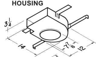
MODEL 503 HOUSING
