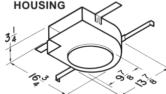
MODEL 502 HOUSING
