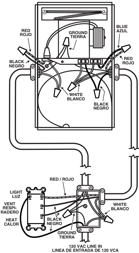
FIG. 10 MODEL 655, 655MX, 659
