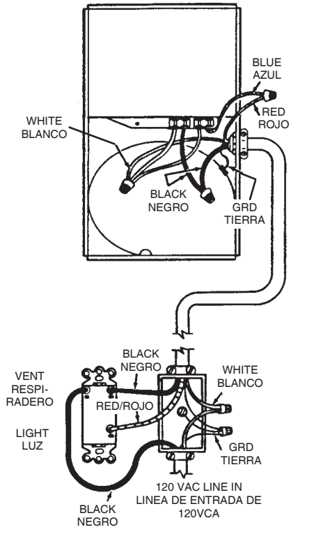
FIG. 11 MODEL 657
