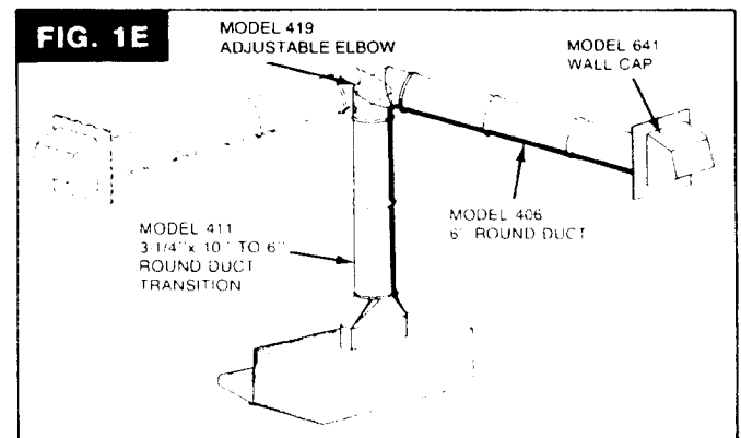
FIG. 1E. Ducting between ceiling joists for multi-story installations or through soffits above cabinets where soffit connects to outside walls.
