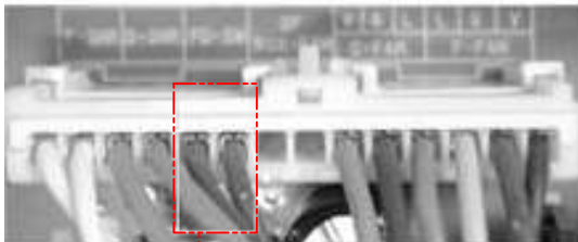
CON7 (PIN5&6) CONNECTOR 7 F-DOOR S/W 2*RD PIN 5&6
