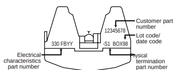
(OVERLOAD PROTECTOR cross section)
