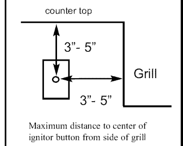
Built-in dimensions using a Trim Kit
