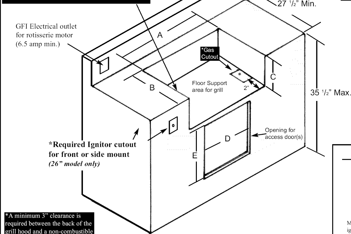
Built-in dimensions without using a Trim Kit
