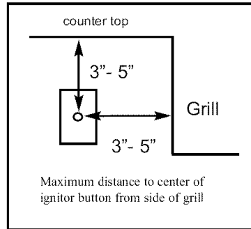
Built-in dimensions using a Trim Kit
