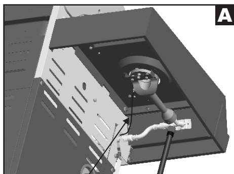
Sideburner Ignitor Wire
