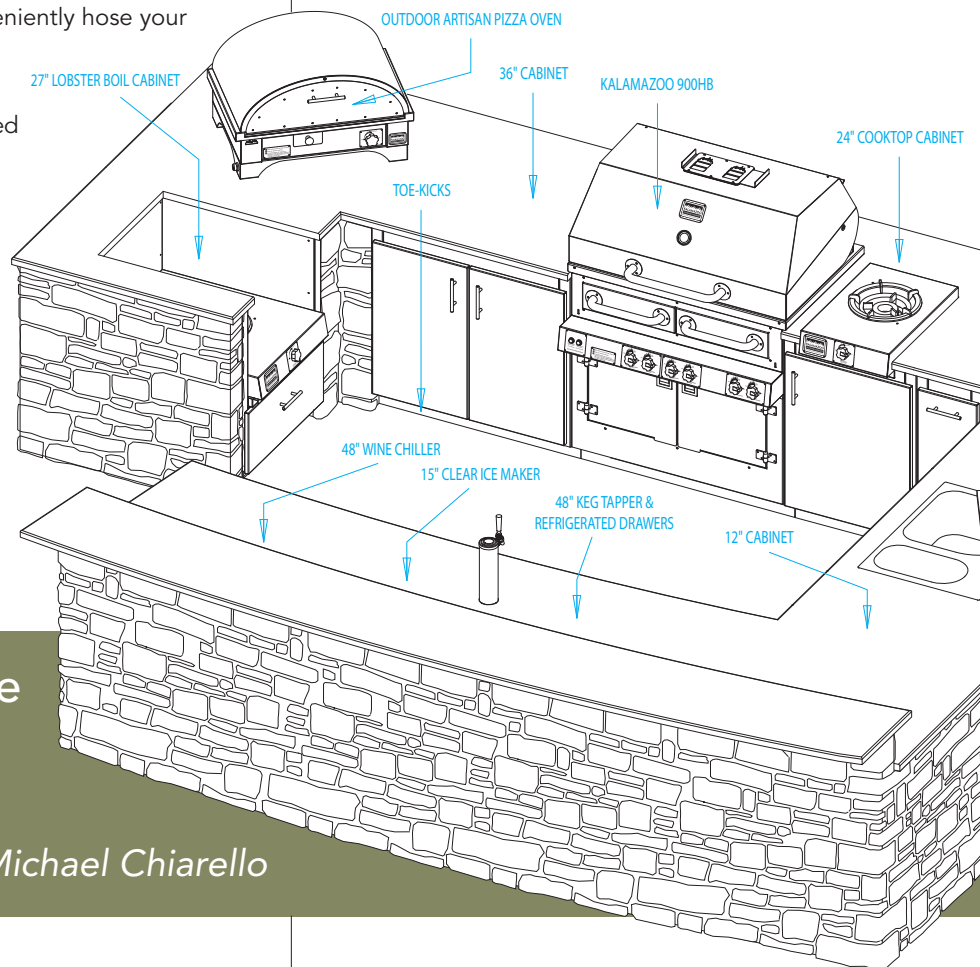
Our weather-tight design features seamless rain gutters around every door and drawer opening. Kalamazoo Outdoor Gourmet cabinets are the only ones to feature all stainless steel hardware, including the slides and hinges.
