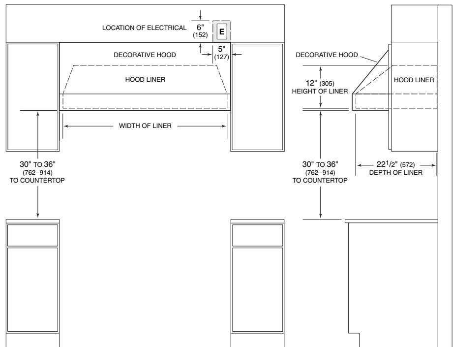
VERTICAL DISCHARGE ONLY FOR VENTILATION HOOD LINERS.
