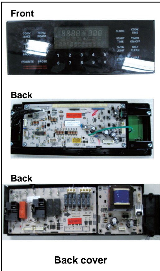
Controller assembly
