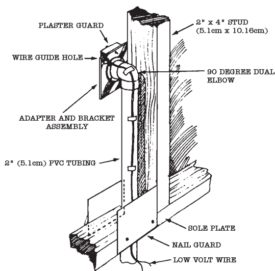
Stud-Mounting Bracket Assembly (New Construction)
