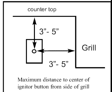
Built-in dimensions using a Trim Kit
