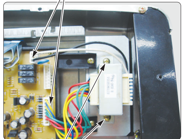
2 Connector
