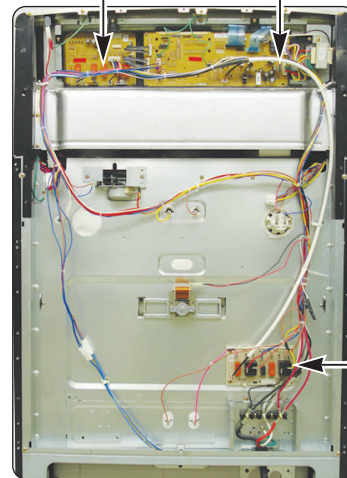
Cook-top Relay PCB Main PCB
