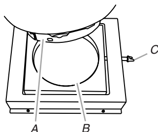
A. Bottom collar B. Mounting hole C. Locking screw
