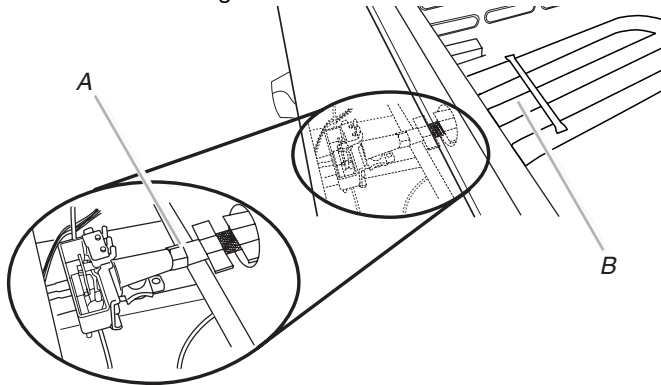
A. Burner/gas orifice connection B. Middle tube of burner
