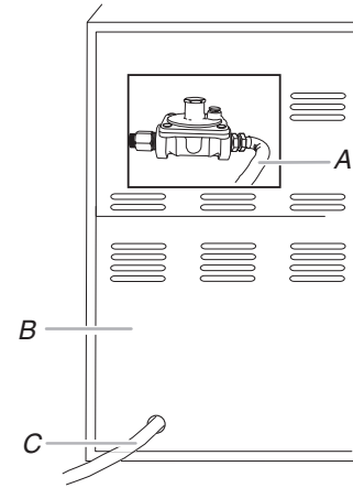
A. New ANSI Z21.54 certified gray hose B. Rear of grill C. To local LP gas supply
