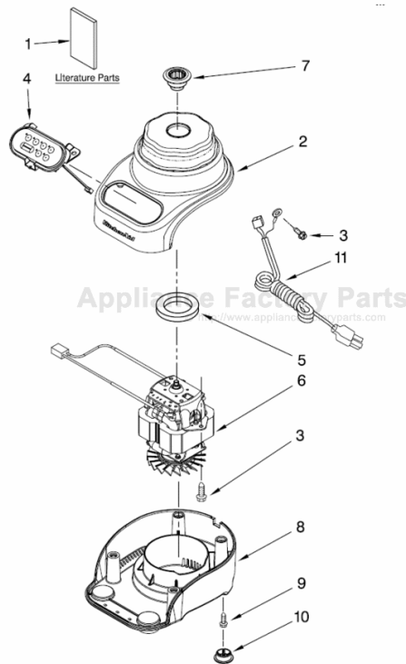
UNIT PARTS FOR VARIATIONS OF MODEL: KSB465_0
