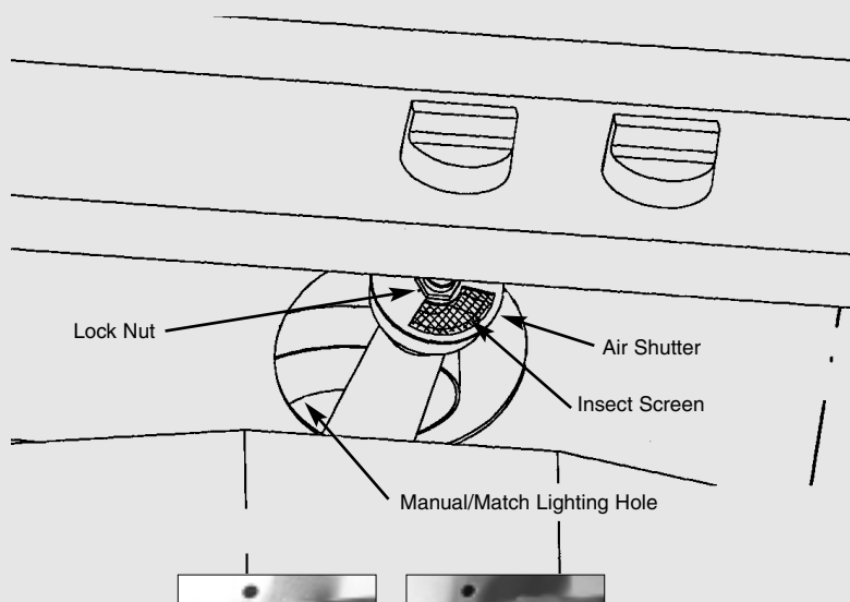
FIGURE 6 CUTAWAY VIEW
