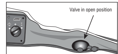
Turn Control dial to DEFLATE position.
